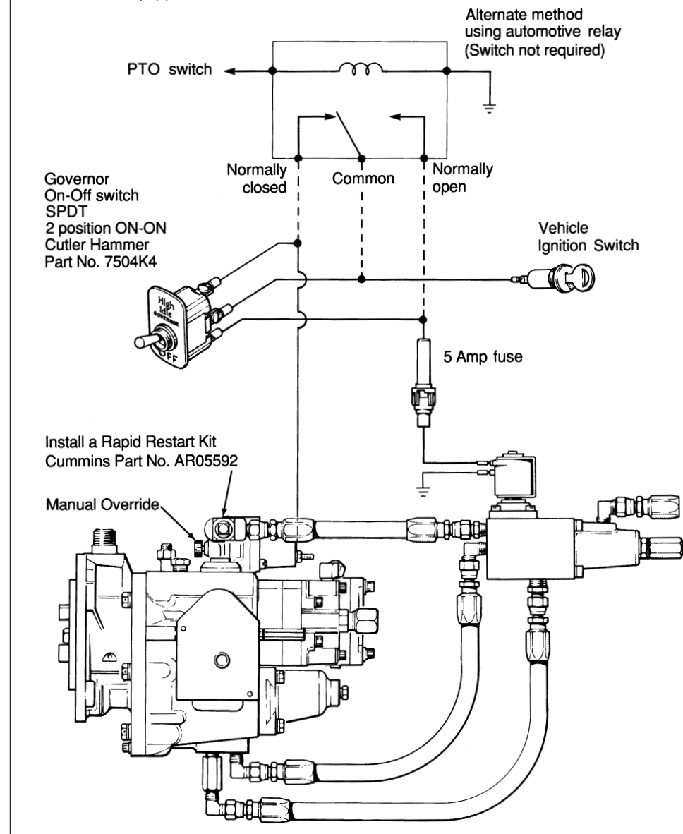
Figure 9: Wiring schematic for throttle lockout on PTO equipped vehicles
