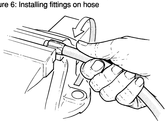
Figure 6: Installing fittings on hose
