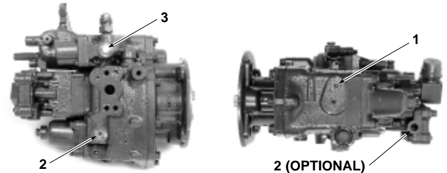
Figure 5: VS Type Pump
